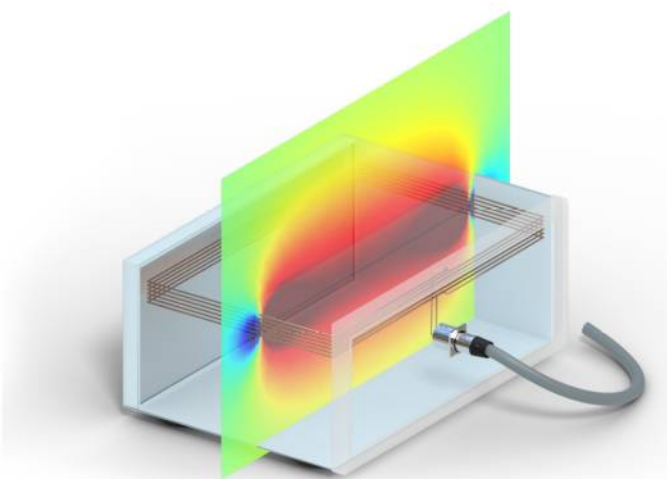
Fig. 17 - The antenna, made by a rectangular and balanced solenoid, is housed in a plastic enclosure. The contour plot, simulated with COMSOL Multiphysics ® , software, shows the computed levels of the magnetic field in the longitudinal-vertical plane.
